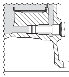
Fig. 7.3 – Drain plug D
