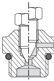
Fig. 7.2 – Vent plug V
