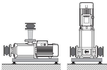
Fig. 6.5 – Example of installation to reduce vibration and noise
