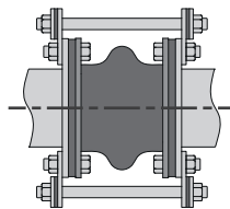
Fig. 6.6 – Example of rubber joint with limiting tie rods
