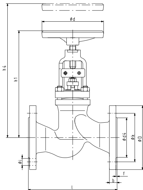
III. 2: Dimensions/Poids NORI 40 ZXLBV
