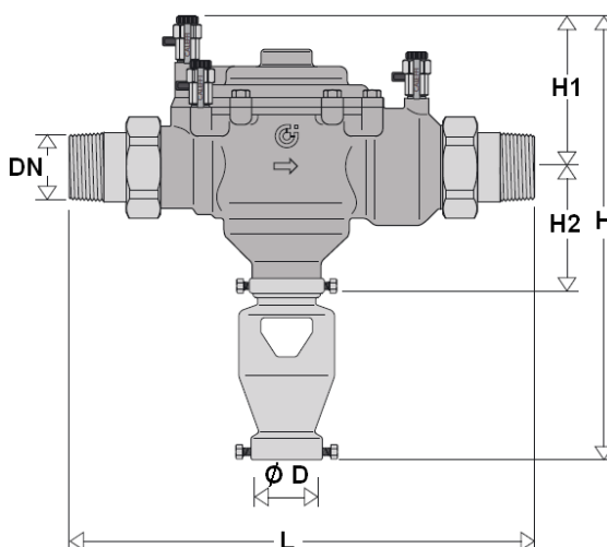
DN 2"
