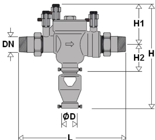
DN 1"1/4 DN1"1/2
