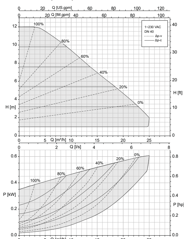
Calio 40-120 \Delta p_v , \Delta p_c
