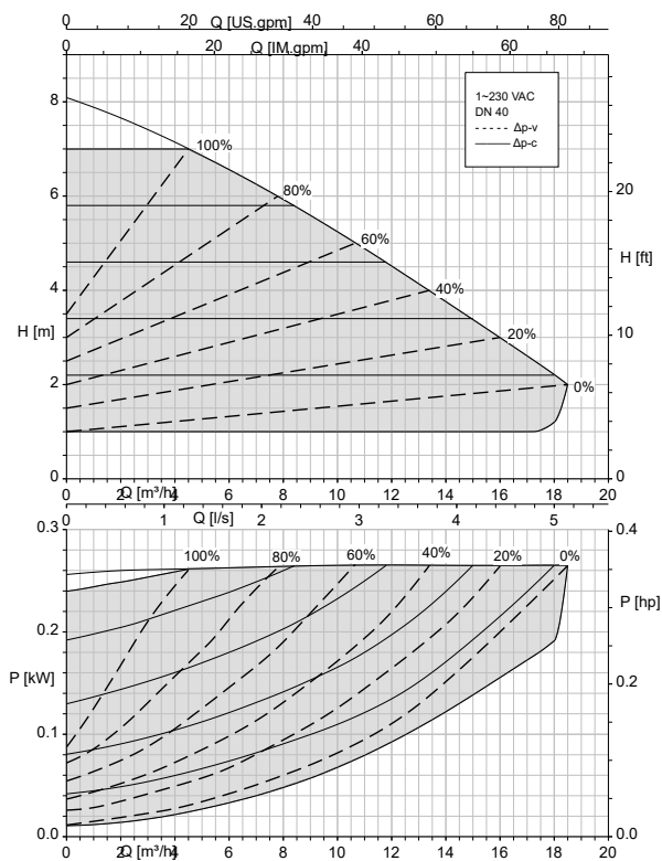
Calio 40-90 \Delta p_v , \Delta p_c
