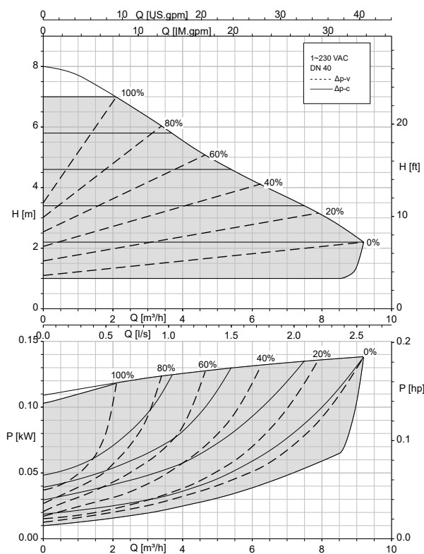
Calio 40-70 \Delta p_v , \Delta p_c
