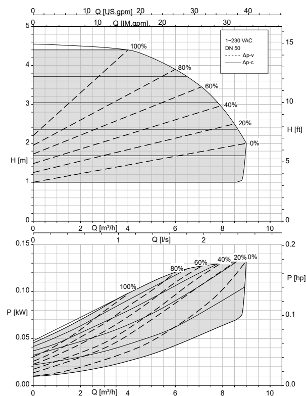
Calio 50-40 \Delta p_v , \Delta p_c
