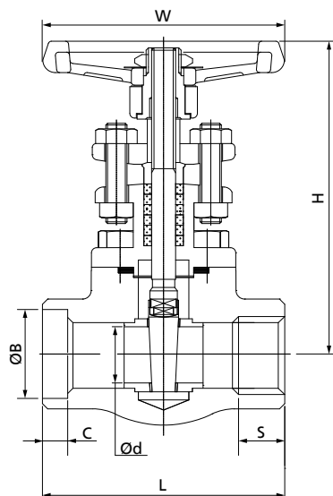
III. 2: Dimensions ECOLINE GTF 800
